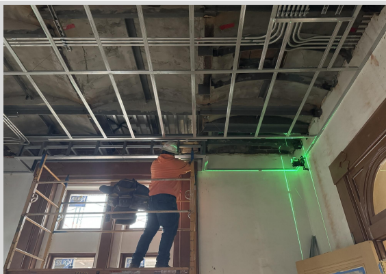
2 nd Floor Ceiling Framing 3/7/25
